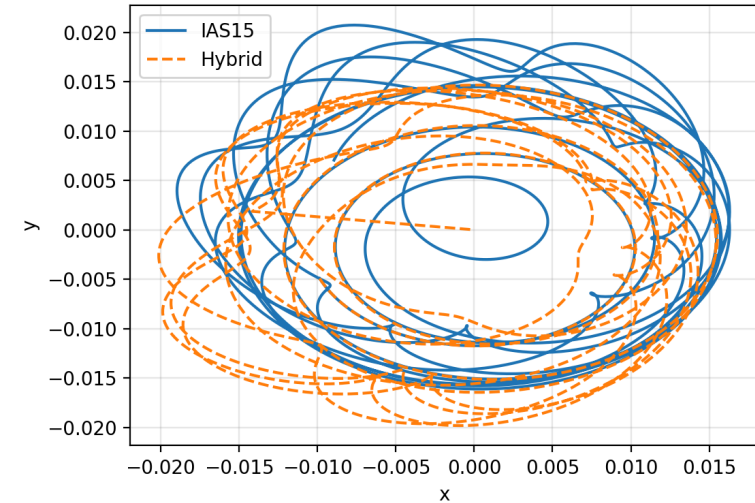
Body 0 XY (T=100 yr)
